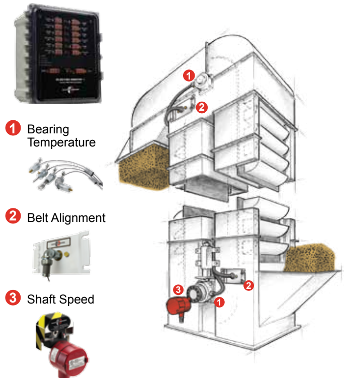
Hazard monitoring on a bucket elevator.
