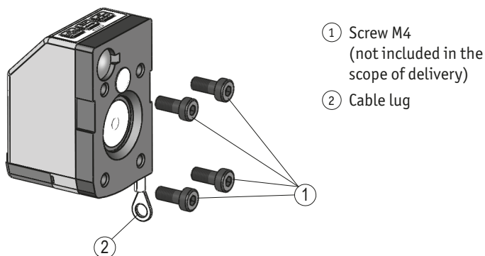
Fig. 2: Mounting
