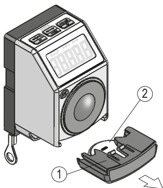
Fig. 4: Battery change
